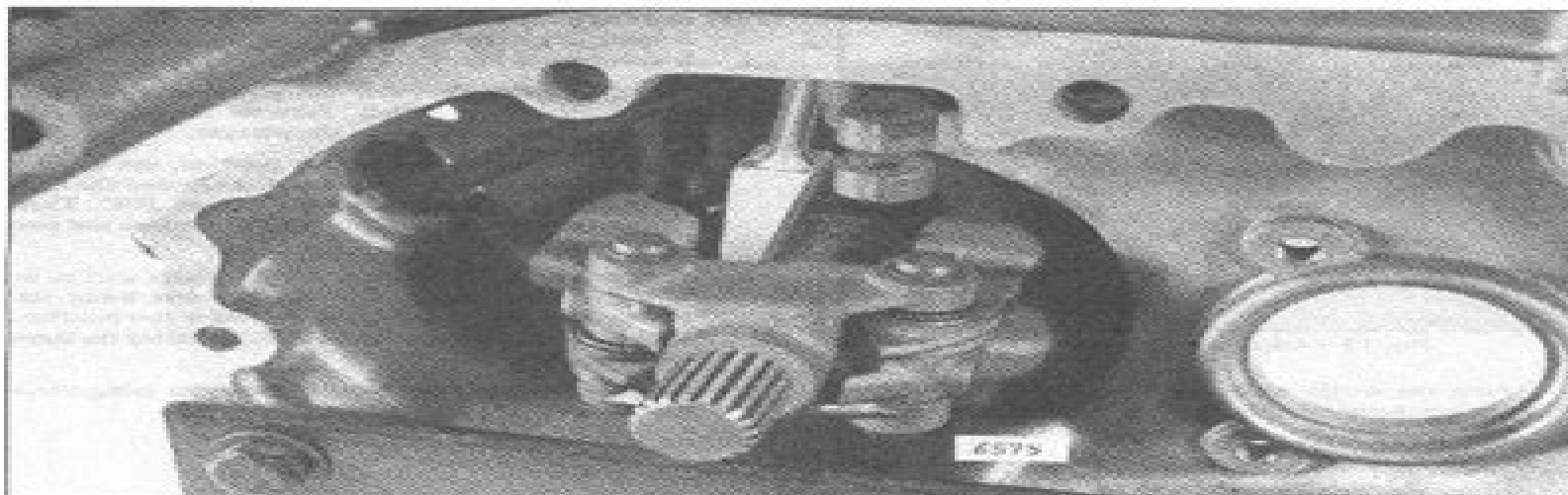
Fig. 13 - Wedge of Tool J35516 Between Riser and Low Speed Weight (Detail)
