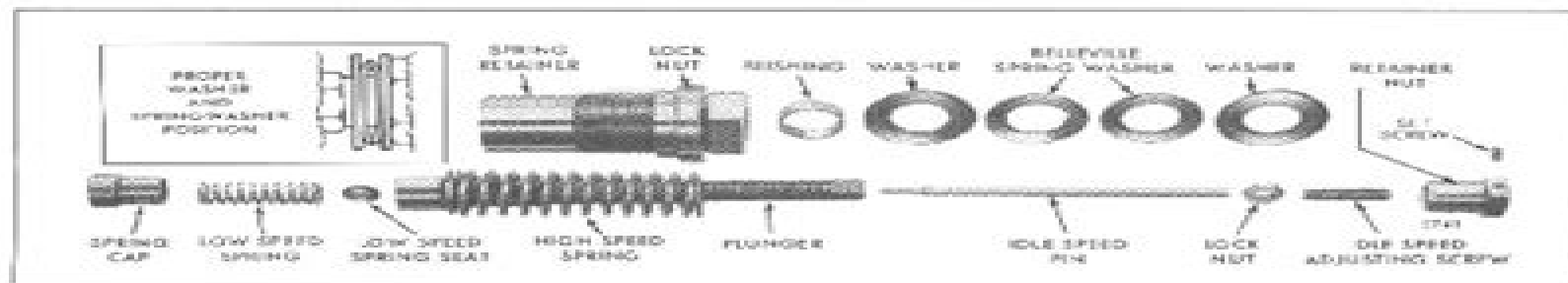
Fig. 14 - High and Low-Speed Springs and Plunger Details Including Belleville Washers (TTA Engine)
