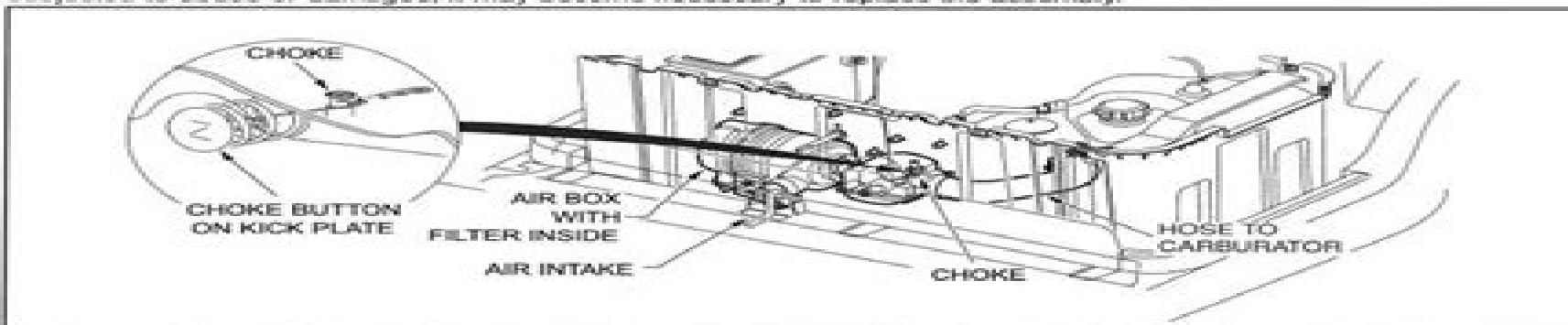
Figure 16-8 Air Intake and Choke Assembly
