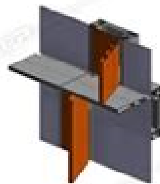
3. INTERMEDIATE MULLION & PANEL, WITH FIN - 3D VIEW
