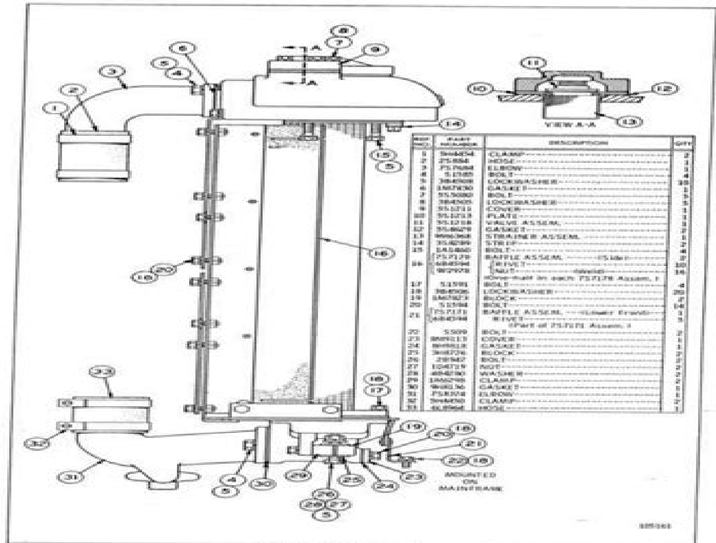
RADIATOR—Side View Refer also to Page 135 for special parts
