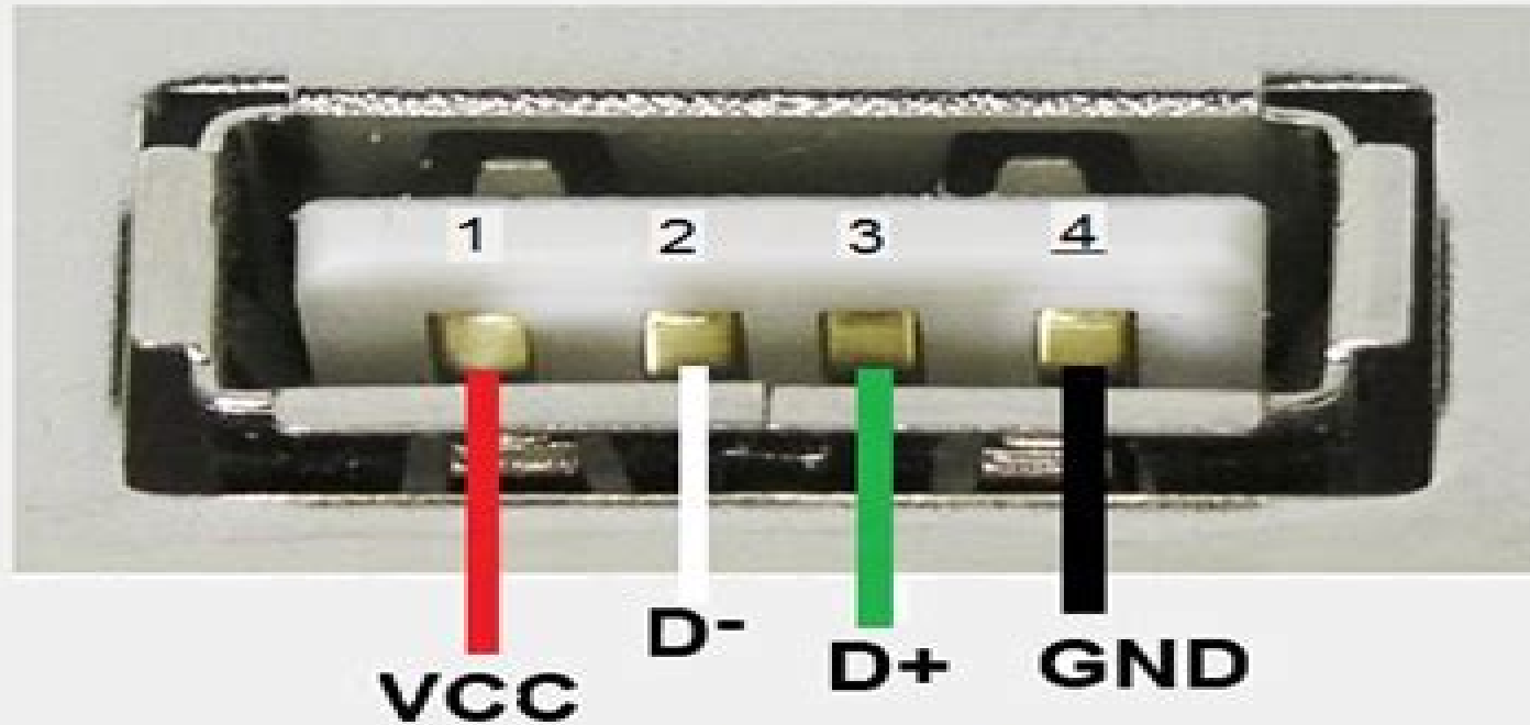
The USB Pinout: front female face
