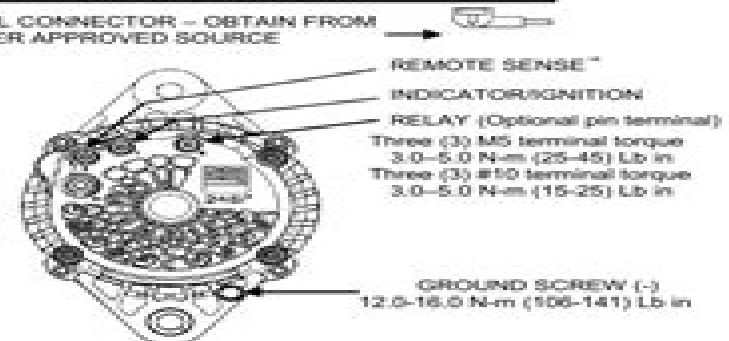
FIGURE 2 - 24SI™ (4-Terminal studs & 3-Terminal studs & Pin)
