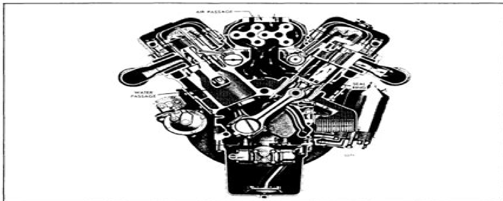
Fig. 5 - Air and Water Passages in 8V Cylinder Block
