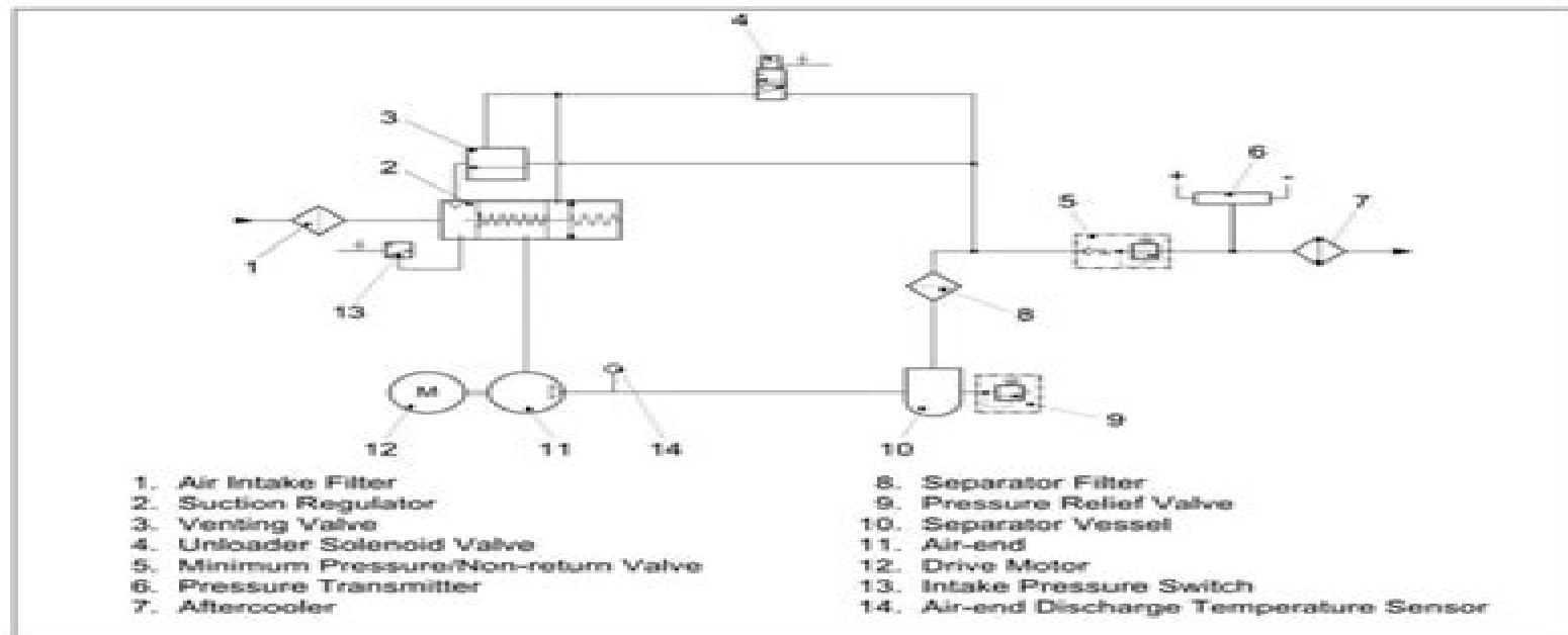
AIR COMPRESSOR CIRCUIT DIAGRAM – ON/OFF CONTROL
