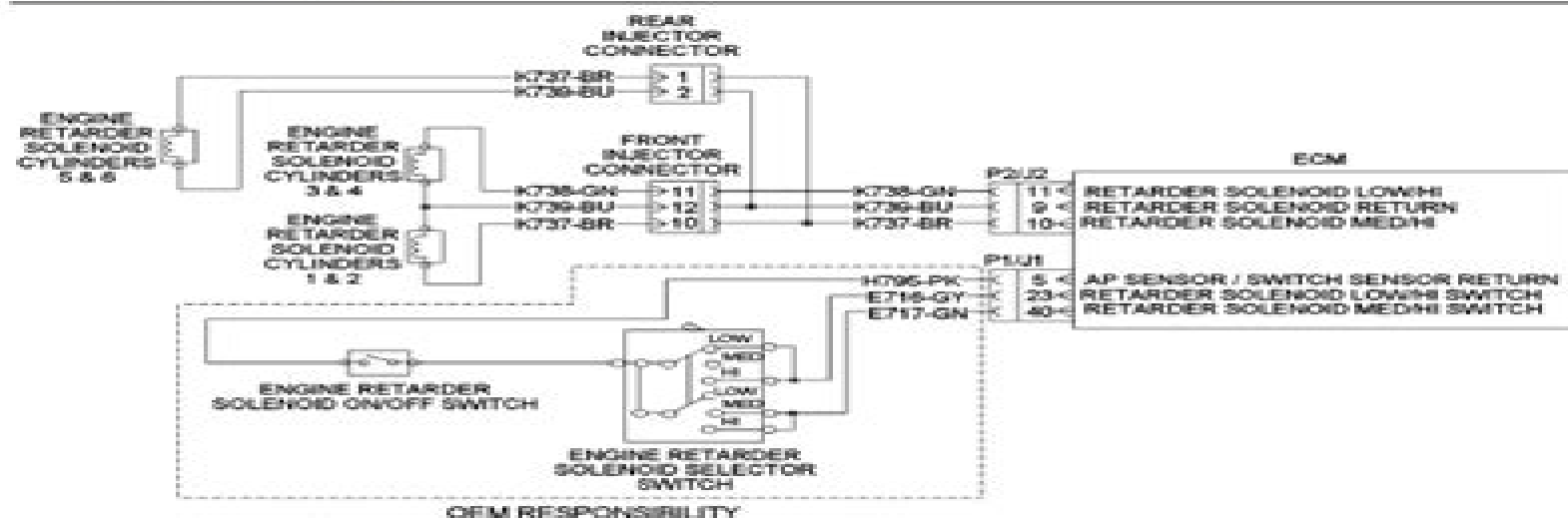
Illustration 170 Schematic for the C15 engine
