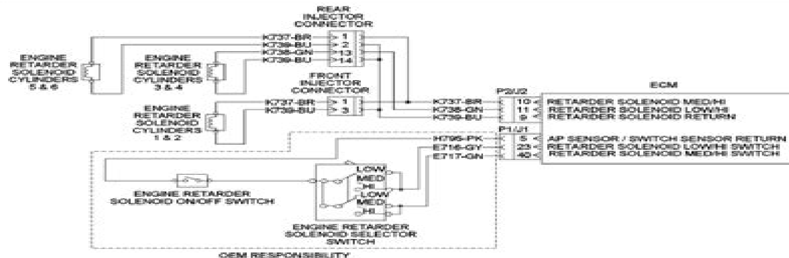
Illustration 169 Schematic for C11 and C13 engines
