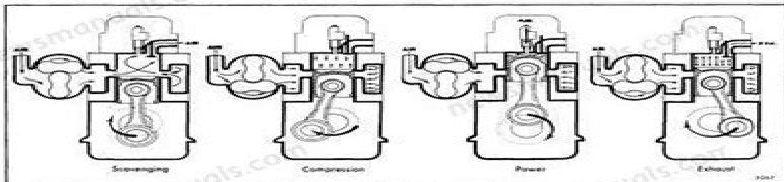
Fig. 1 - The Two Stroke Cycle
