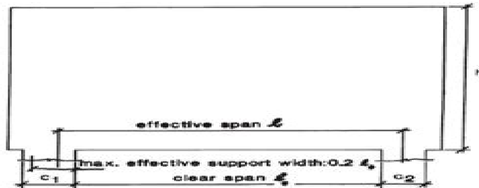
Figure 1.2 CIRIA Guide 3—meanings of symbols c_1 , c_2 , h , l and l_e
